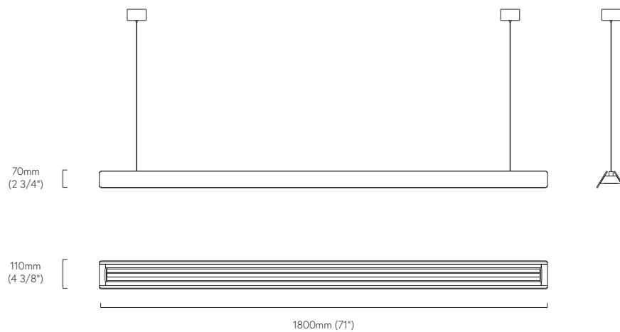
WEDGE 1800mm
