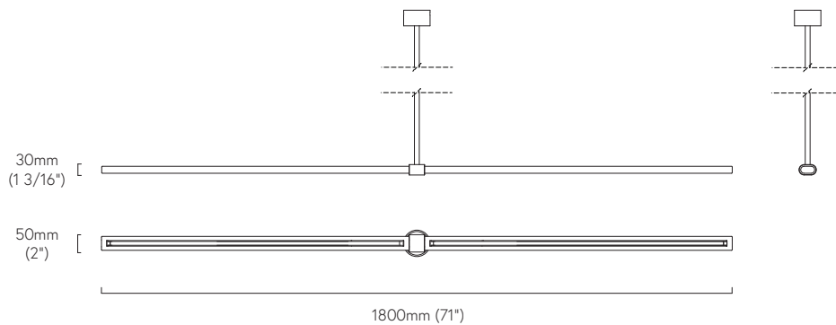
SPRIG 1800mm
