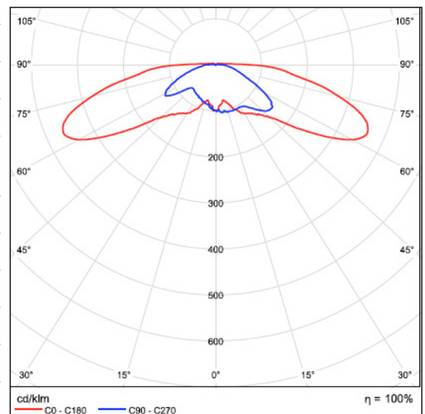
Light distribution (at 18W)
